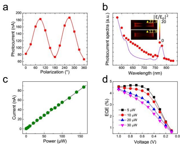
Figure 3. Photo response characteristics of the vacuum channel nanoscale diode. (a) Photocurrent polarization dependence during device excitation at \lambda=633 \text{ nm} . Angle 0^\circ of polarization is parallel to the long axis. (b) Theoretically calculated absorption spectra (purple line) and experimentally measured photocurrent spectra (red points) of the device at polarizer angle 0^\circ (parallel to the long axis). Inset: electromagnetic field distribution of the device extracted from the purple line in Figure 3b. The maximum of |E/E_0|^2 is 22.3 and 12.9 at \lambda=780 \text{ nm} (top) and \lambda=710 \text{ nm} (bottom), respectively. (c) Photocurrent for the representative device as a function of input laser power (Au electrode biased to -1 V). (d) Plot of the measured external quantum efficiency (EQE) as a function of applied voltage for different input laser power.
