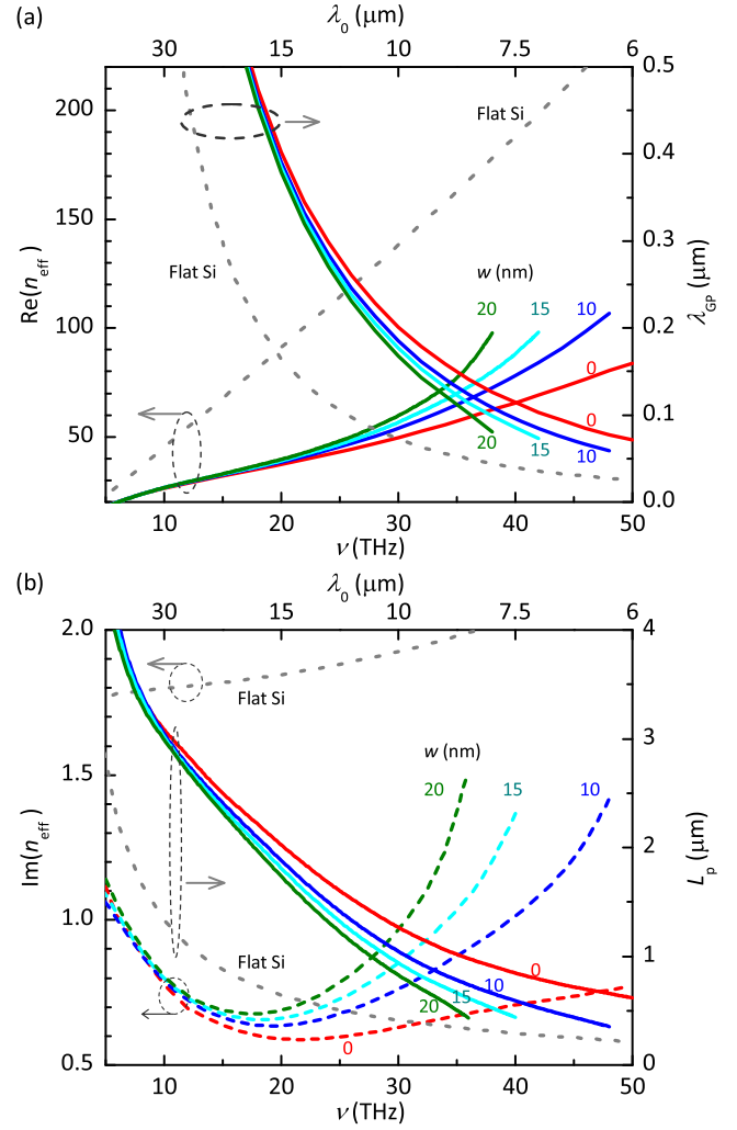
Fig. 2. Dispersion of GPs on silicon, corrugated silicon ( w = 10, 15, 20 \text{ nm} ) and substrate of SAPL (denoted by w = 0 ). Thickness of corrugated layer is h = 100 \text{ nm} . (a) Real part of effective refractive index (left axis) and GP wavelength (right axis) with respect to photon frequency. (b) Imaginary part of effective refractive index (left axis) and propagation length (right axis) with respect to photon frequency.
