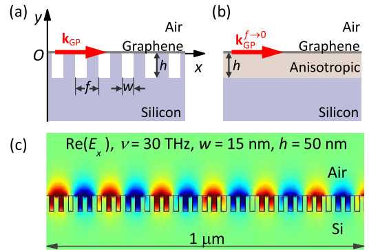
Fig. 1. (a) Configuration of plasmonic waveguide consisting of a graphene sheet on silicon penetrated by an array of air grooves. (b) Effective structure of short array period limit (SAPL, f/\lambda_{GP} \rightarrow 0 ), where the anisotropic layer has the same thickness as the air grooves, with its permittivity given by Eq. (1). (c) Snapshot of longitude electric field at frequency of 30 THz, assuming w = 15 nm, h = 50 nm, f = 2w and graphene Fermi level of 0.4 eV.
