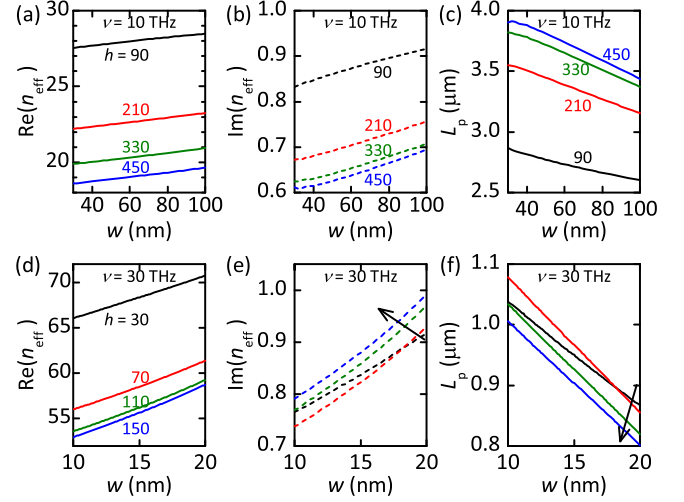
Fig. 3. Effective refractive index n_{\text{eff}} and propagation length L_p in terms of air groove width w , with fixed air groove thicknesses h . (a) and (d) Real part of n_{\text{eff}} . (b) and (e) Imaginary part of n_{\text{eff}} . (c) and (f) Propagation length. In (a)–(c), \nu = 10 THz. In (d)–(f), \nu = 30 THz. Along the arrows in (e) and (f), h = 30, 70, 110, 150 nm.
