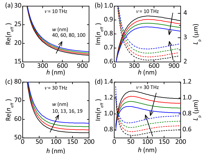
Fig. 4. Effective refractive index and propagation length in terms of corrugated layer thickness, with fixed air groove widths. (a) and (c) Real part of n_{\text{eff}} . (b) and (d) Imaginary part of n_{\text{eff}} (dashed) and propagation length (solid). In (a) and (b), \nu = 10 THz, w = 40, 60, 80, 100 nm along the arrows. In (c) and (d), \nu = 30 THz, w = 10, 13, 16, 19 nm along the arrows.
